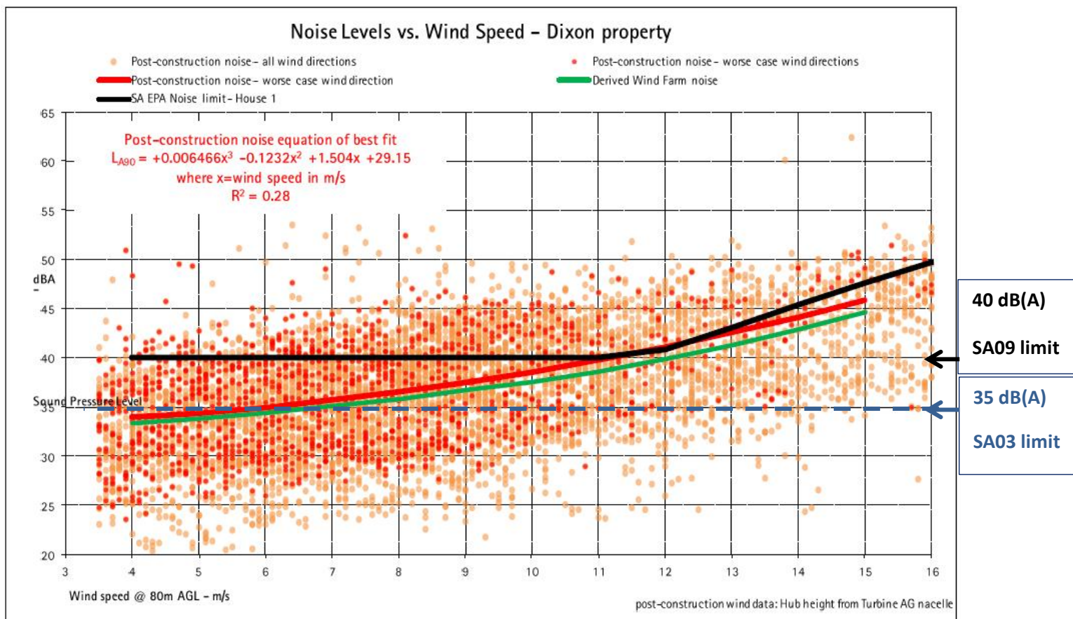
Figure 3: Post-construction noise levels vs. wind speed at the Dixon property
